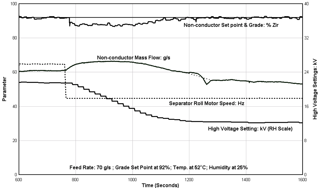
Figure 8: Grade control with speed change of separation roll
