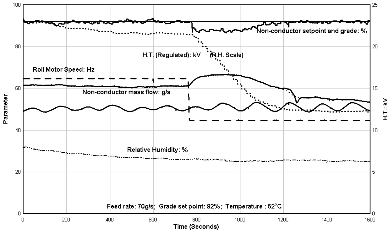
Figure 10: Grade control with variations in humidity and roll speed
