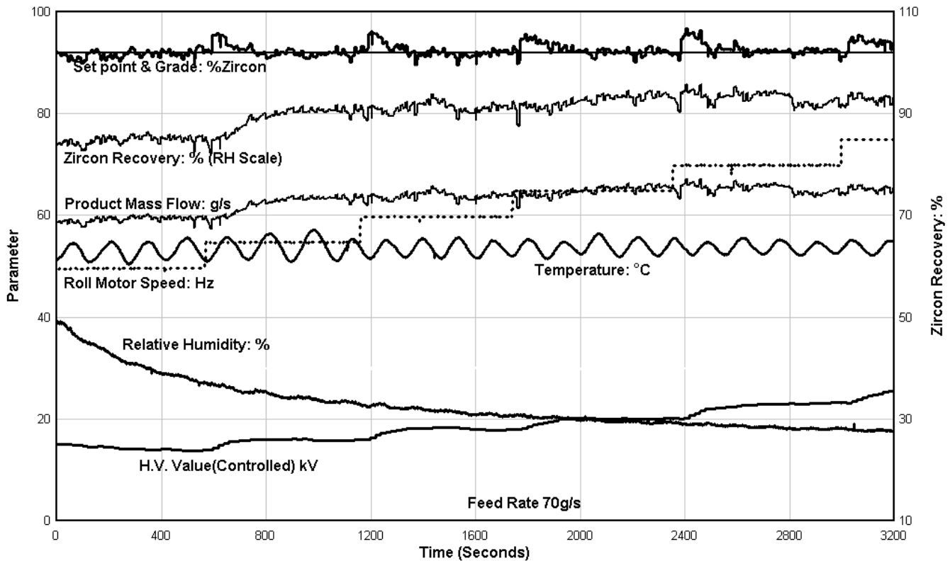
Figure 12: Settings optimised for maximum recovery
