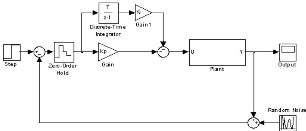
Figure 7: Control system for the pilot plant
