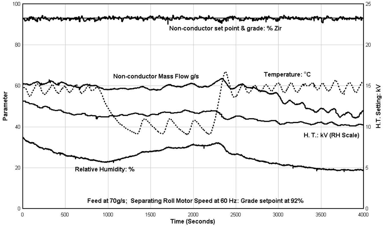
Figure 9: Grade control with varied humidity and roll speed
