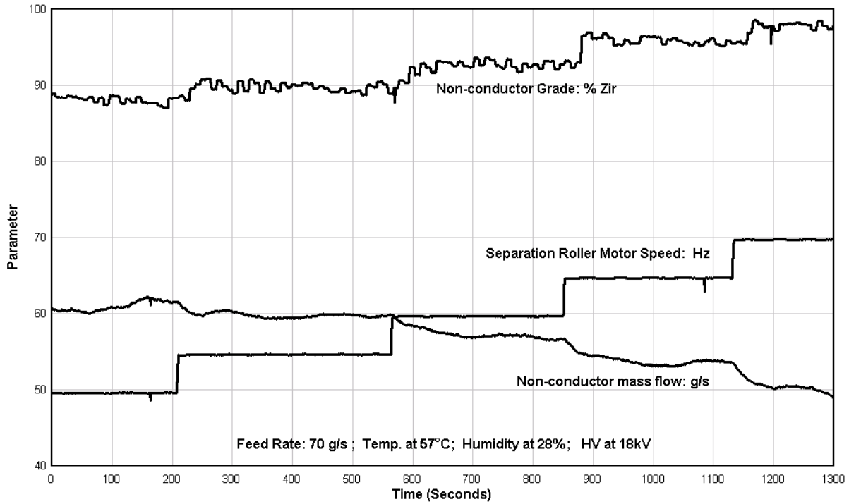
Figure 4: The impact of roll speed on separator performance
