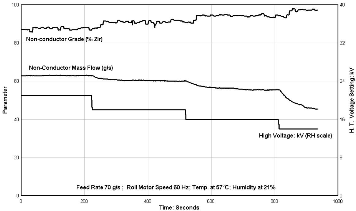
Figure 5: Impact of voltage settings on separator performance
