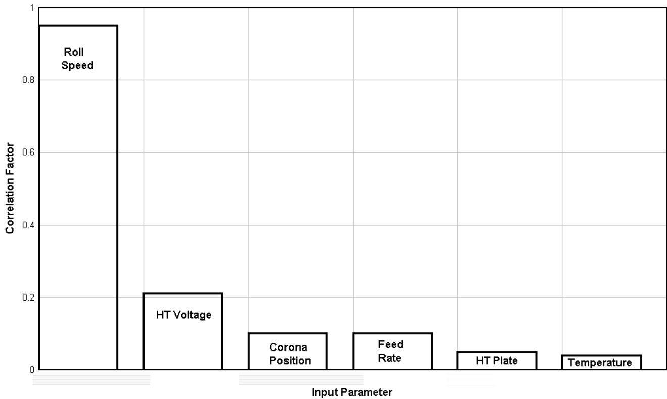
Figure 3: Impact of various factors on product grade
