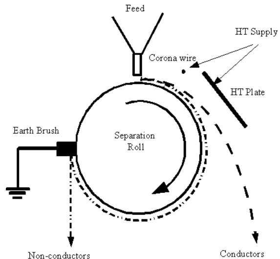
Figure 1: Schematic of a High Tension Roll Separator
