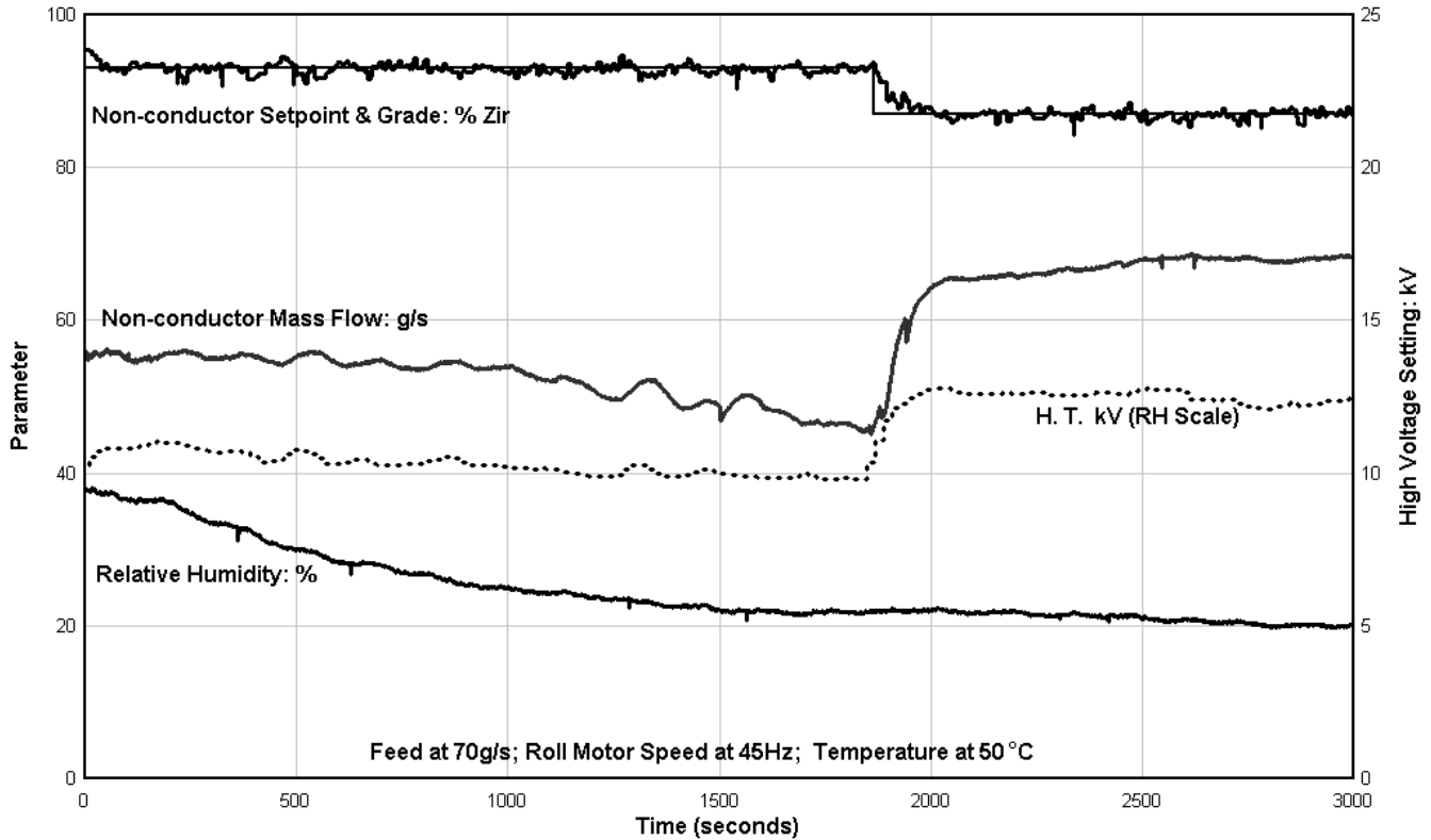
Figure 11: Control with a change in humidity and a change in set point
