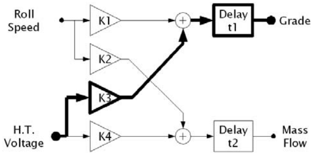
Figure 6: Basic plant model
