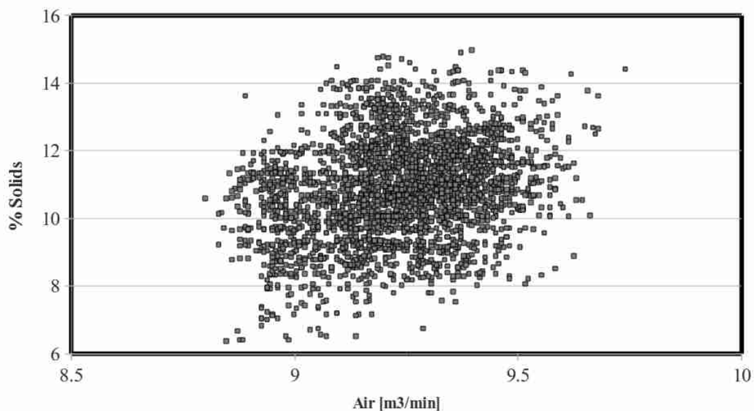
Figure 2.1 Response of % Solid to Air addition
