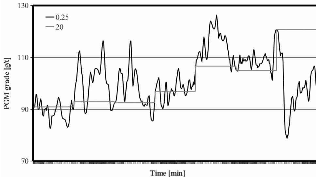
Figure 5.6 PGM data: 15 seconds and 20 minutes
