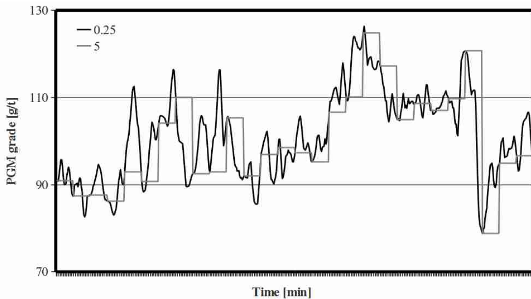
Figure 5.4 PGM data: 15 seconds and 5 minutes
