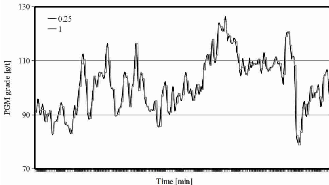
Figure 5.3 PGM data: 15 seconds and 1 minute
