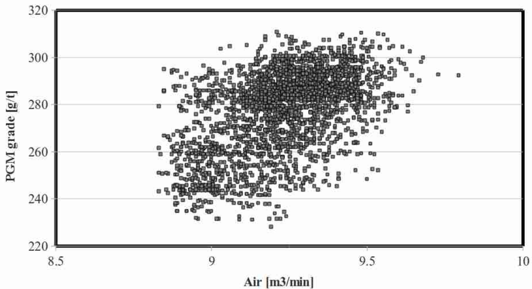
Figure 2.2: Response of PGM grade to Air addition
