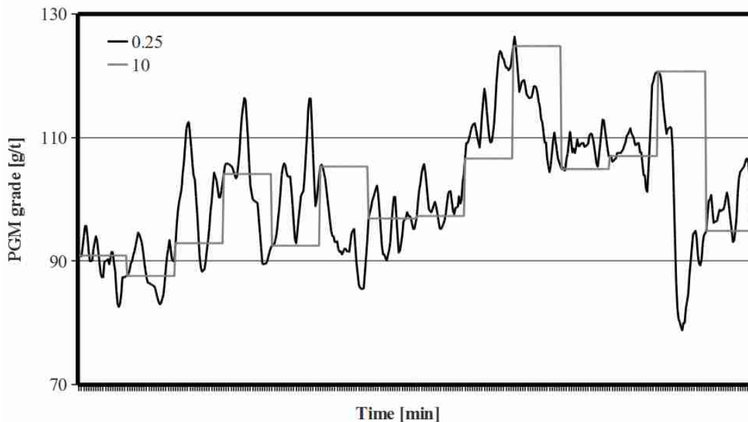
Figure 5.5 PGM data: 15 seconds and 10 minutes
